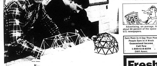
The Carline Mercury/Heather Mathis News Photo Josh Abnapp, left, and Mike Jolly work on engineering structures in dome and bridge construction as part of Jim Simons' Industrial Technology class.
