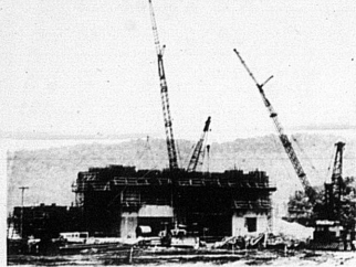
Construction progresses at the new Charleston Bottoms Power Station on Highway 8 near Mayville with much of the effort being devoted to building the bases of the turbine-generator and the stack. Completion of this East Kentucky (Wichester) Power Cooperative station is scheduled for 1976.—Jerry Schreman photo.
