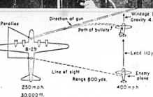
Upper plane shows the central gunner's control system of a B-29 Superfortress, which was demonstrated publicly for the first time in New York city...
