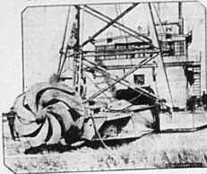
View of the monster bi-rotary dredger being used to cut the ship and power canal between Lakes St. Louis and St. Francis on the St. Lawrence river. The dredger is being used to get around the rapids there. The bar dredger cuts 200 feet of earth daily and will soon complete the canal which will be 300 feet wide and 17 feet deep. The canal is part of the St. Lawrence waterway.
